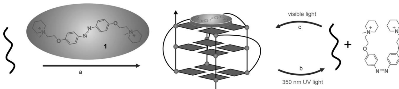
Figure 3. Reversible folding and stretching motion of the G quadruplex was induced by the photoresponsive compound 1: a) the telomere DNA was induced to form a G quadruplex; b) the folded G quadruplex was disassociated by irradiation with UV light at 350 nm for 1 min (stretching); c) the stretched oligomer folded into the G quadruplex again upon illumination with visible light for 1 min (folding).
