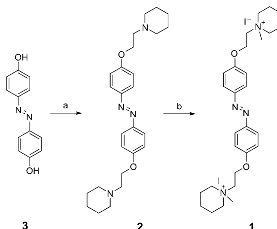
Scheme 1. Synthesis of compound 1 : a) 1-(2-chloroethyl)piperidine hydrochloride, dry acetone, K 2 CO 3 , argon, reflux, 59%; b) CH 3 I, CHCl 3 , 45 °C, 49%.
